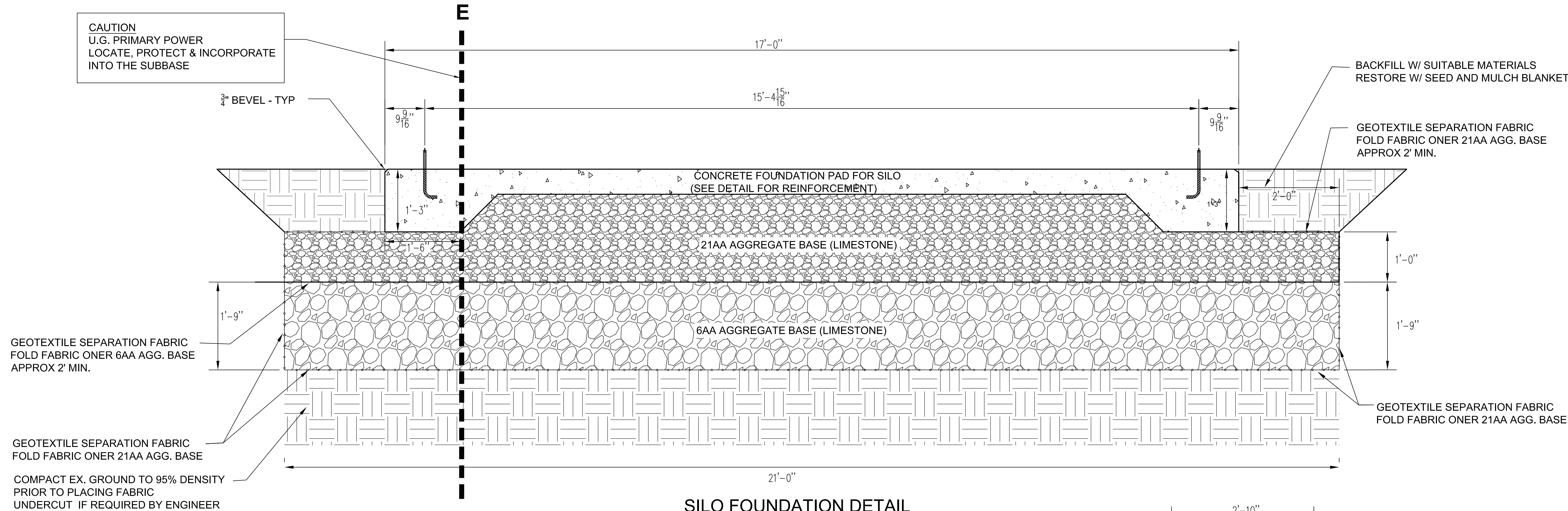
SILO FOUNDATION DETAIL
