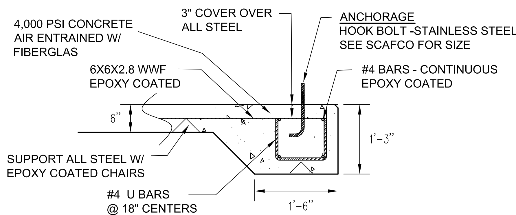
SILO FOUNDATION DETAIL
