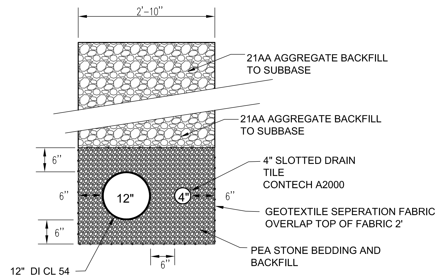
STORM SEWER REPLACEMENT DETAIL
